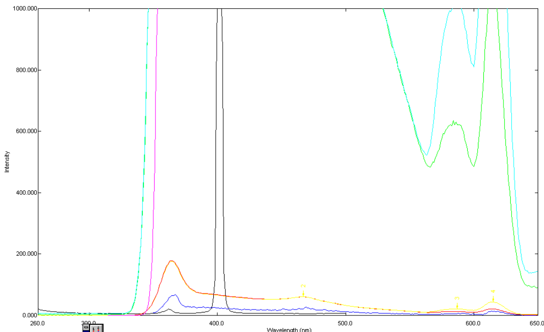
Fig.4: Photoluminescence of BaMgAl 10 O 17 -Eu (0.5%), BaMgAl 10 O 17 -Eu (1.0%), BaMgAl 10 O 17 -Eu (1.5%)
