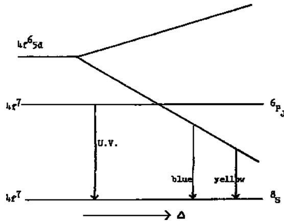
Fig.3: The energies of 4f^7 and 4f^6 5d^1 levels in \text{Eu}^{2+} influenced by crystal field
