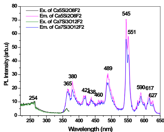
Fig.6: Excitation and Emission spectra of \text{Ca}_5\text{Si}_2\text{O}_8\text{F}_2 & \text{Ca}_7\text{Si}_3\text{O}_{12}\text{F}_2 at 1200°C
