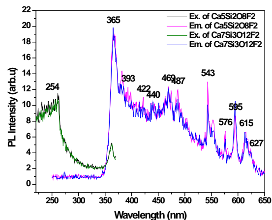
Fig.2: Excitation and Emission spectra of \text{Ca}_5\text{Si}_2\text{O}_8\text{F}_2 & \text{Ca}_7\text{Si}_3\text{O}_{12}\text{F}_2 at 900°C
